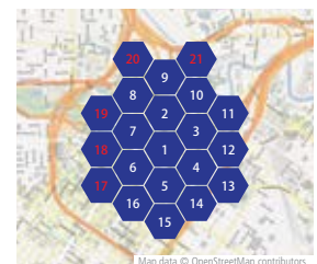
12.5 kHz digital system At a total of 2150 sq. miles coverage: 5.8-mile radius per site / 21 site total
